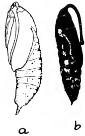
Fig. 32. pupae: a, leaf roller, Coccia rosaceana (Harris); b, tobacco hornworm, Protoperce quinque-maculata Howorth.
